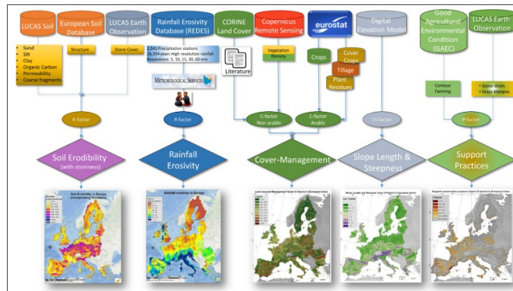
Figure 2.3.2.1 – Soil loss by water erosion ( \text{t ha}^{-1} \text{yr}^{-1} ) in the EU and RUSLE input framework.
