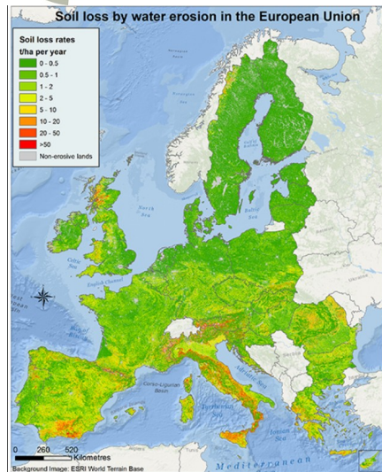
Figure 2.3.2.1 – Soil loss by water erosion ( \text{t ha}^{-1} \text{yr}^{-1} ) in the EU and RUSLE input framework.
