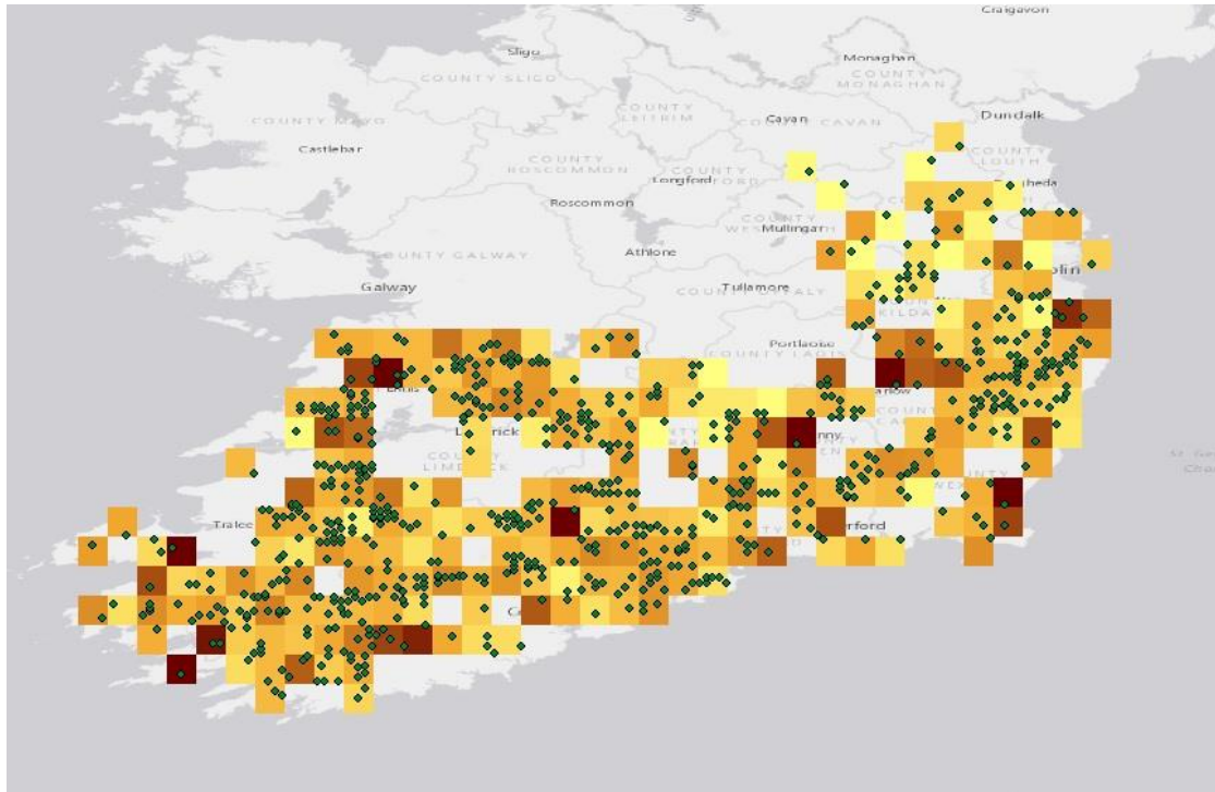
Figure 18: Grid values are based on the average of the available forest plots per grid cell, with varying number of plots per cell.
