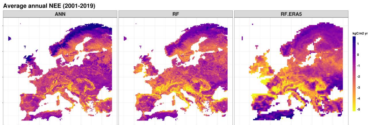
Figure 30: Average annual NEE for the ‘RS+meteo’ setup using ERA5 meteorology as well as the ‘RS only’ setup for two different machine learning methods (random forest and neural networks) for the years 2001-2019.
