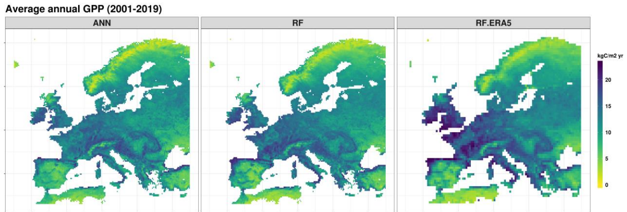
Figure 29: Average annual GPP for the ‘RS+meteo’ setup using ERA5 meteorology as well as the ‘RS only’ setup for two different machine learning methods (random forest and neural networks) for the years 2001-2019.
