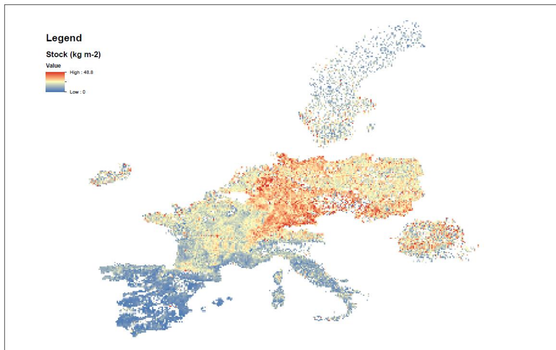
Figure 19: Pattern of forest carbon stocks over Europe over the simulated countries ( \text{kg C m}^{-2} ).
